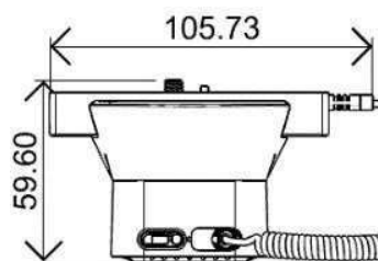
Left view
