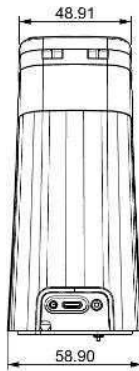
Back view
