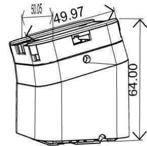
Protection sensor
