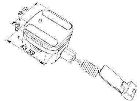
Protection sensor
