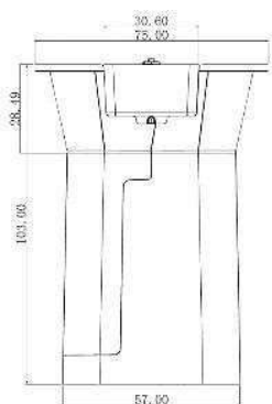
Left view
