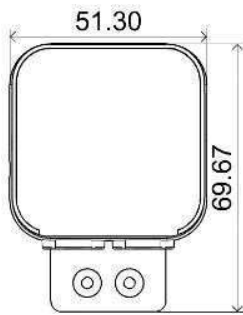
Left view
