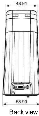
Back view
