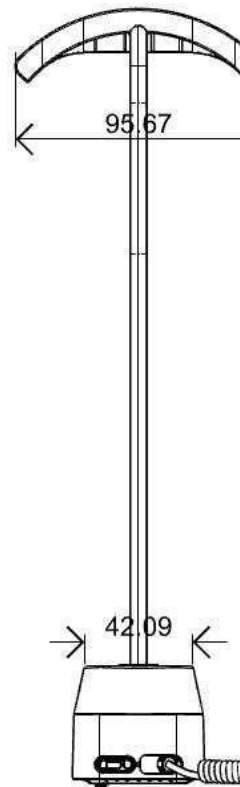
Left view
