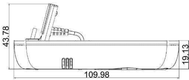
Left view
