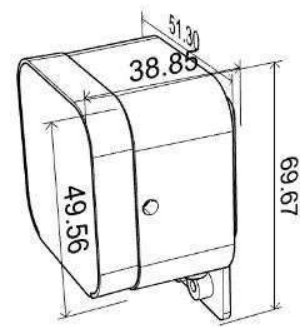
Protection sensor
