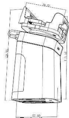
Protection sensor
