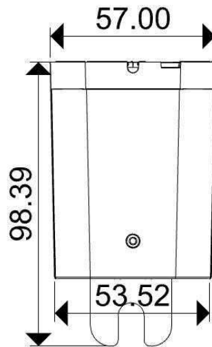
Back view
