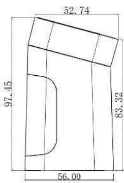
Left view
