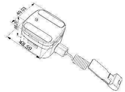
Protection sensor
