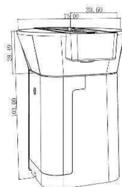
Protection sensor
